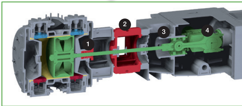
Cylinder with shrunk in, o-ring free, liners.
